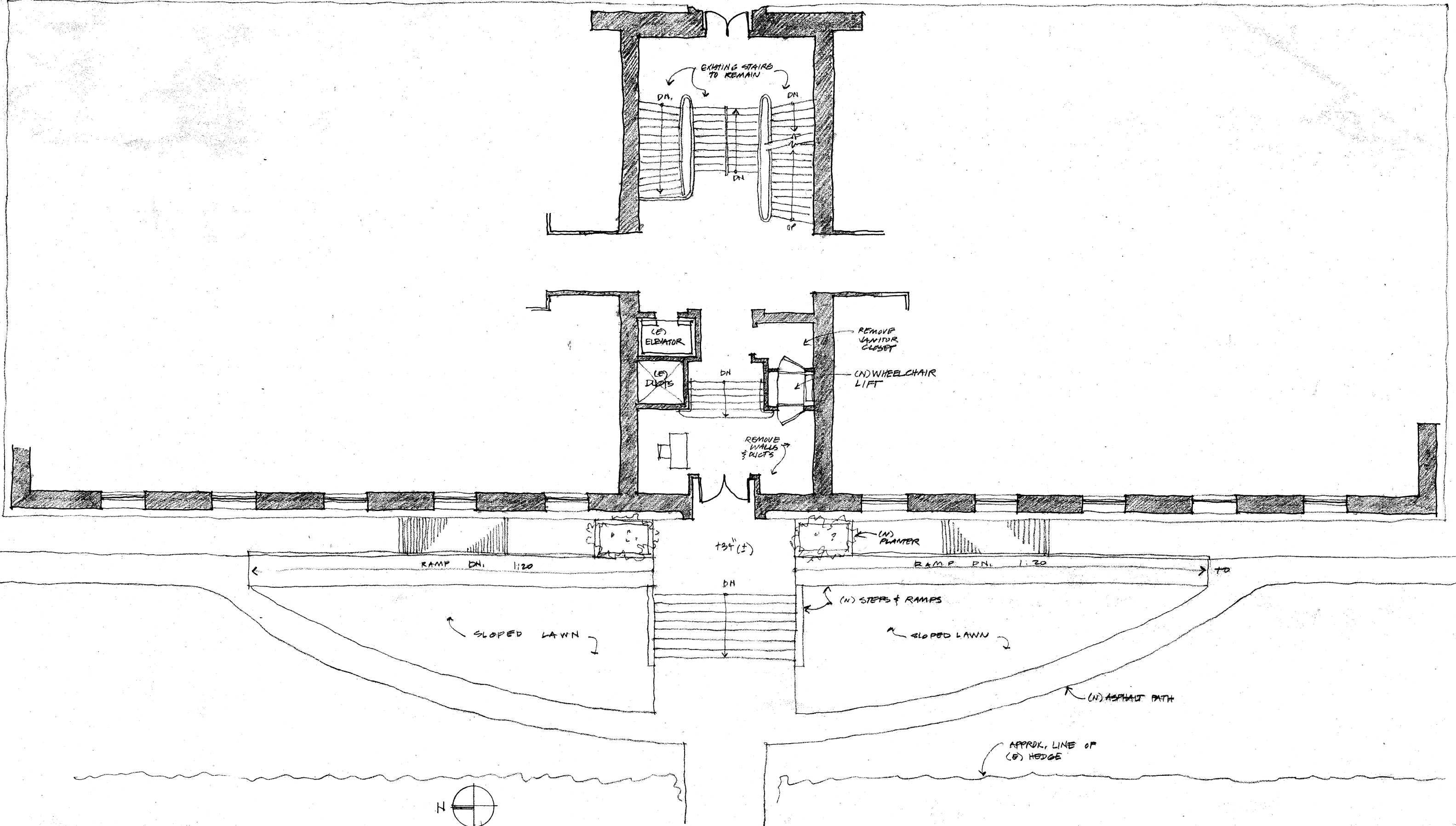
PARTIAL FIRST FLOOR PLAN - OPTION 3 1/8" = 1'-0" JSWD 9.14.07 CALIFORNIA HALL FEASIBILITY STUDY
